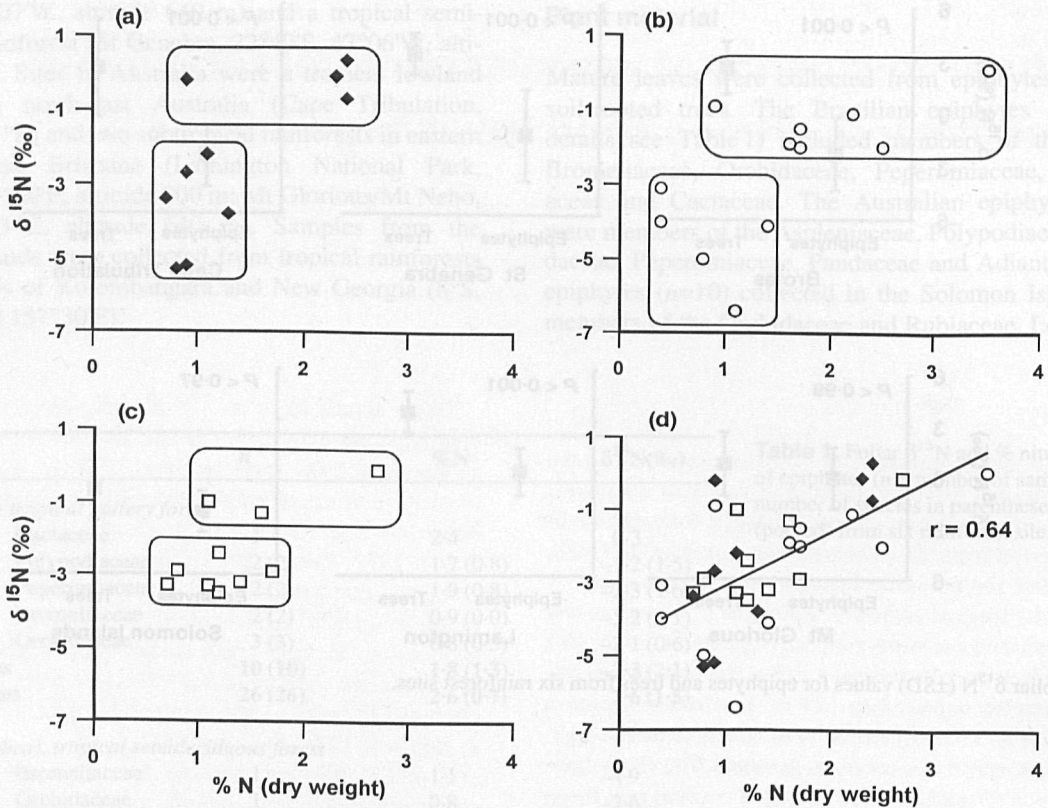
Figure 2. Foliar \delta^{15}\text{N} values and leaf nitrogen contents (% dry weight) for epiphytes from three rainforests: Brotas (a), Cape Tribulation (b) and the Solomon Islands (c) indicating groupings of epiphytes with both low \delta^{15}\text{N} and %N or both high \delta^{15}\text{N} and high %N. Groupings were determined according to Kruskal–Wallis ANOVA by ranks. The data are pooled in (d) and the regression of \delta^{15}\text{N} on %N is shown.
